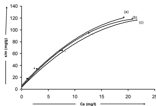
Figure 2. Adsorption isotherms of CN - on Alumina at different temperatures: (a) 283K, (b) 313K, (c) 323K.
