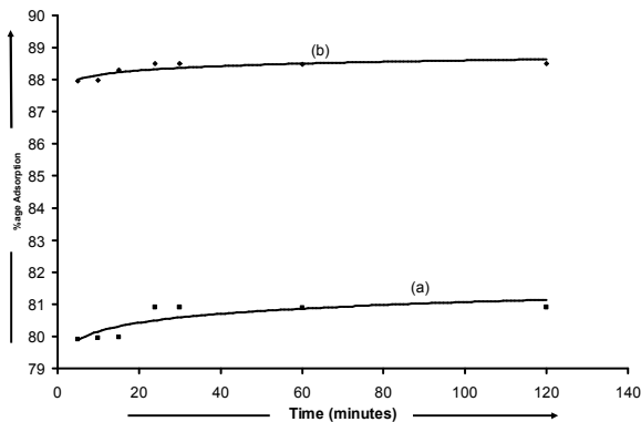
Figure 1. Effect of shaking time on %age Adsorption at (a) 10ppm, (b) 40 ppm for CN - adsorption on Alumina.
