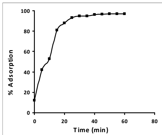
Figure-2. Effect of contact time for the adsorption of endosulfan onto peach nut shells.
