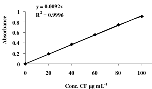
Figure 4. Calibration curve of Ceftriaxone 0.1% using 4-dimethyl aminobenzaldehyde as derivatizing reagent
